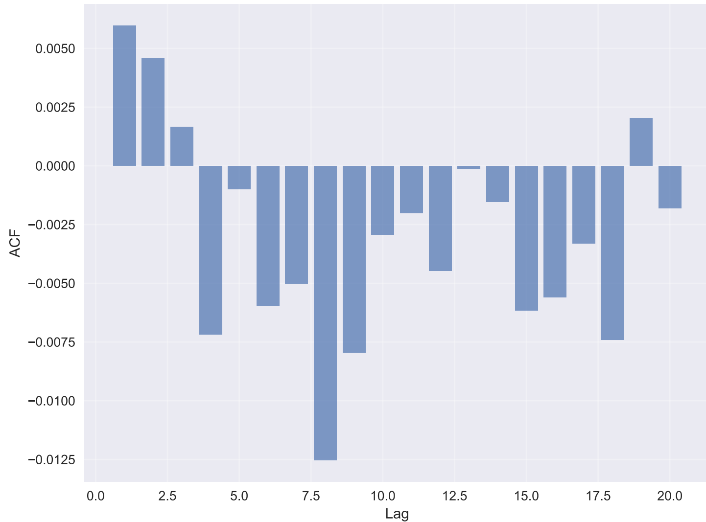
Explicit Conditioned: Volatility Clustering (ACF)
