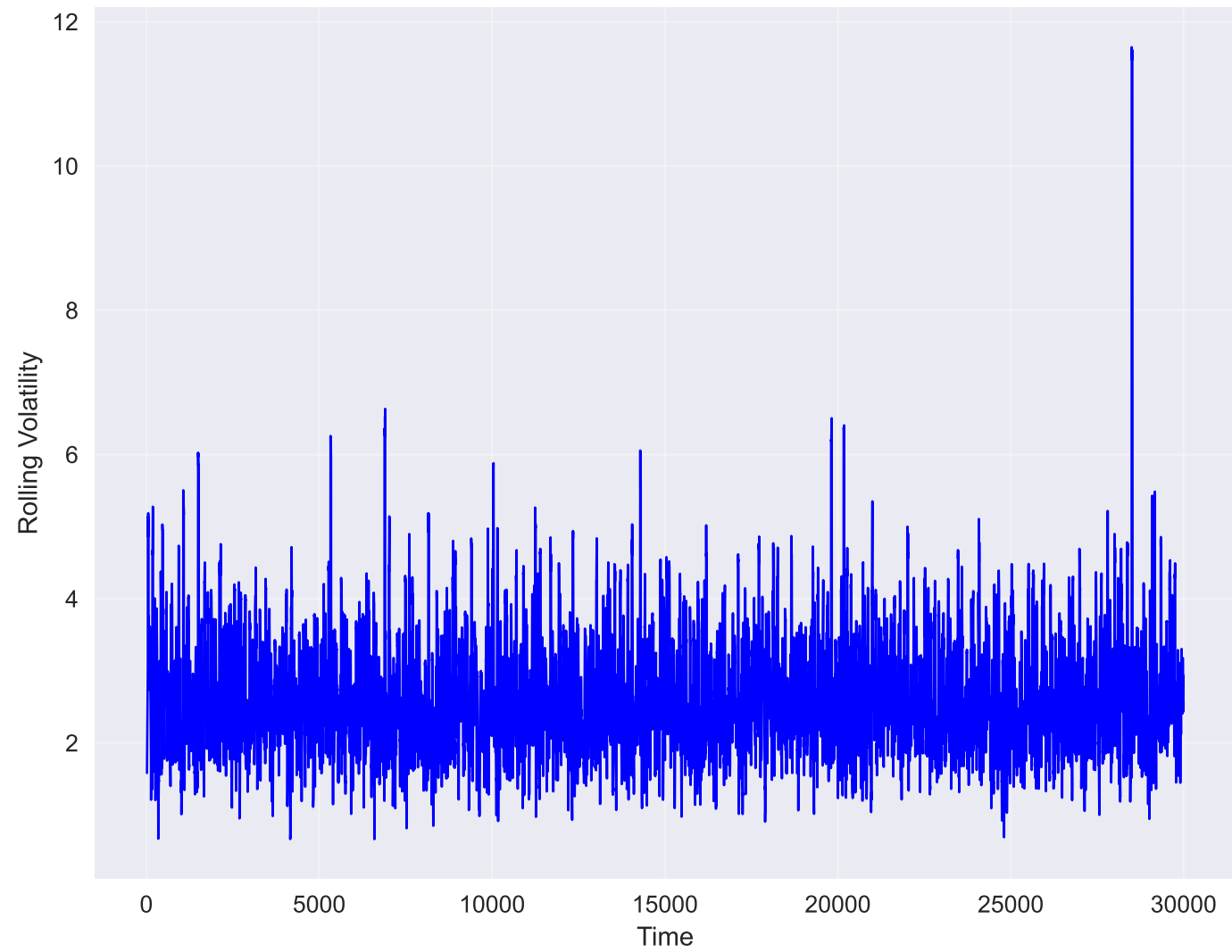
Explicit Conditioned: Rolling Volatility
